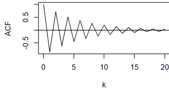
ACF of AR(1): a = -0.85
