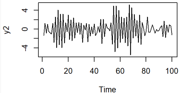
AR(1): a = -0.85
